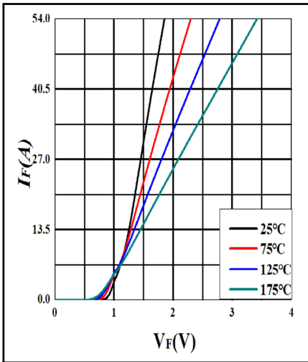
Figure 1. Forward characteristics
