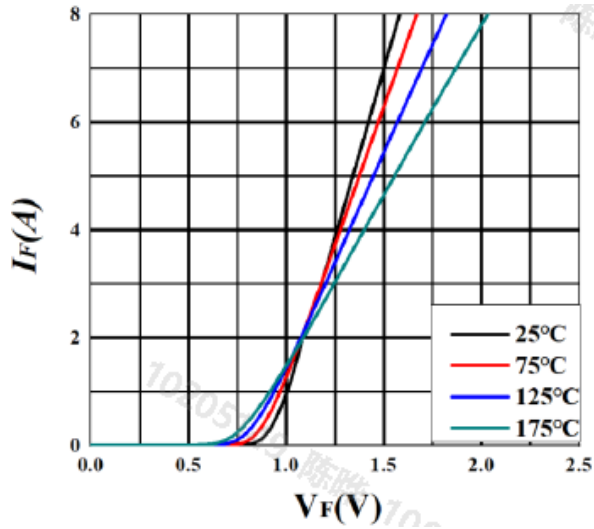
Figure 1. Forward characteristics
