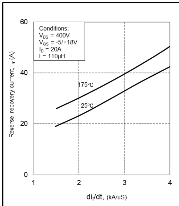
Figure 26. Reverse recovery current vs. di/dt
