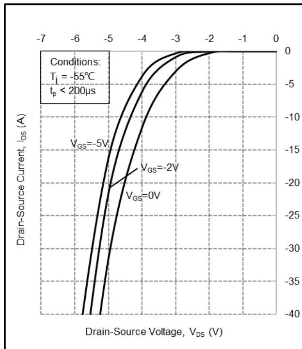
Figure 8. Body diode characteristic at T_j = -55^\circ C
