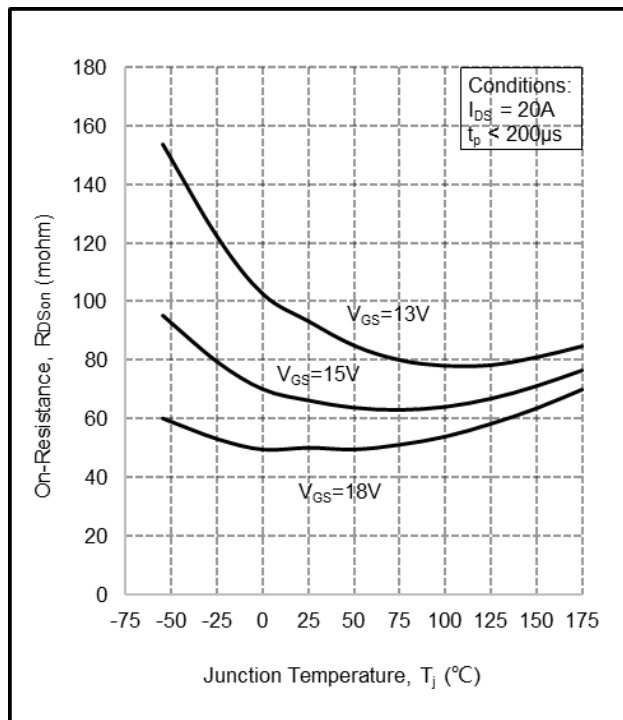
Figure 6. On-resistance vs. temperature for various gate voltages
