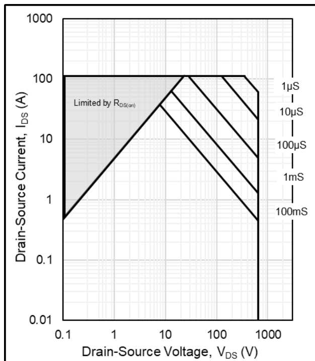
Figure 28. Safe Operating Area
