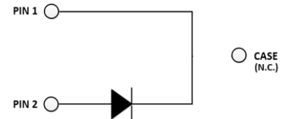
Package Type: TO-220F-2L
