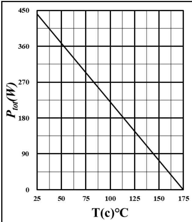
Figure 5. Power derating
