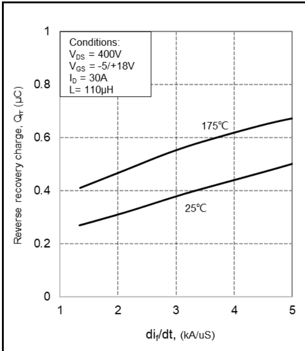
Figure 25. Reverse recovery charge vs. di_r/dt
