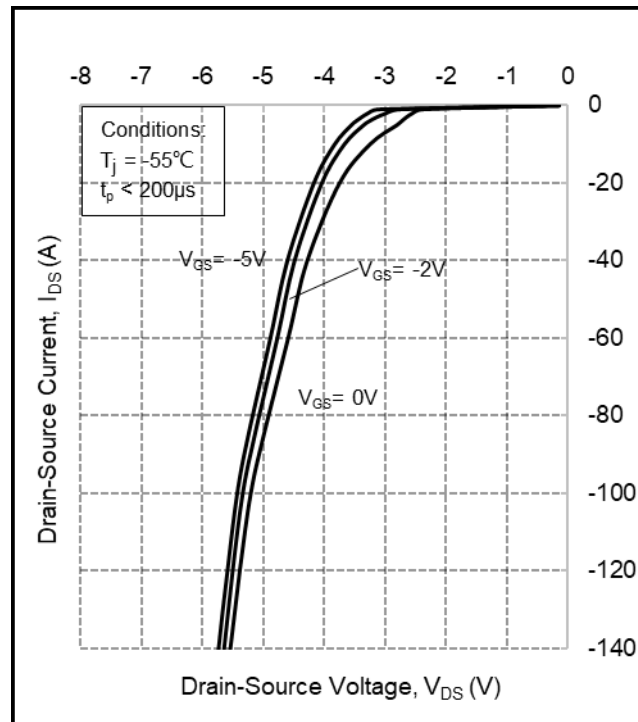
Figure 8. Body diode characteristic at Tj = -55°C
