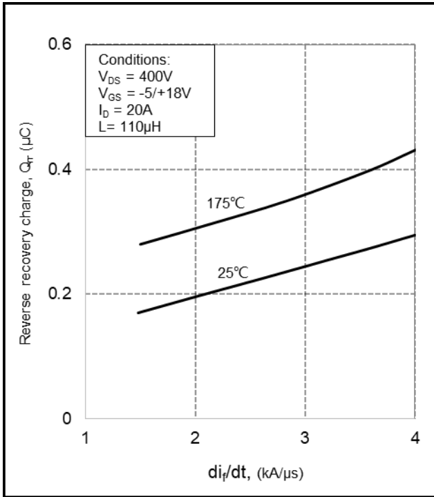
Figure 25. Reverse recovery charge vs. di_r/dt
