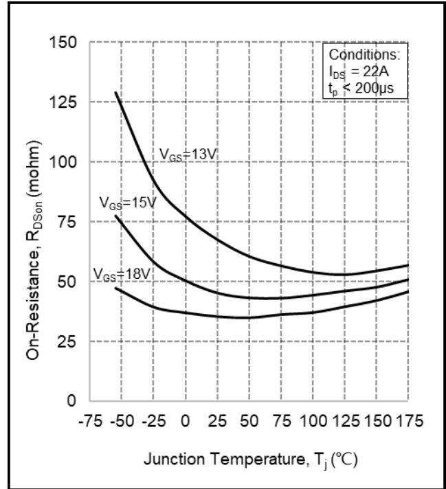
Figure 6. On-resistance vs. temperature for various gate voltages
