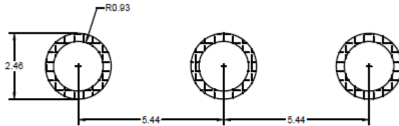
TO-3PF-3L
