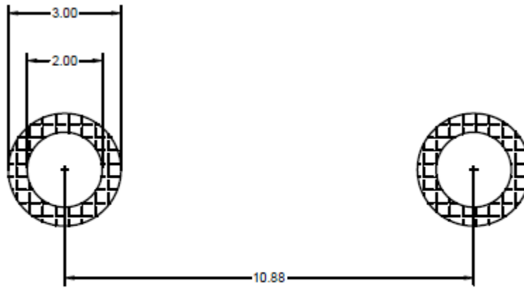
TO-247-2L
