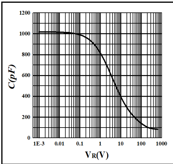
Figure 3. Capacitance vs. reverse voltage
