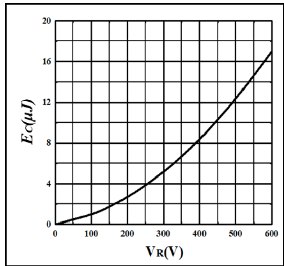
Figure 4. Capacitance stored energy
