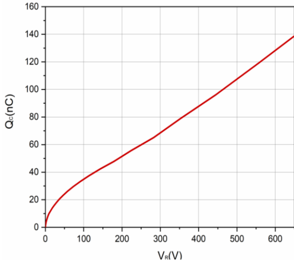
Figure 5. Total capacitance charge vs. reverse voltage
