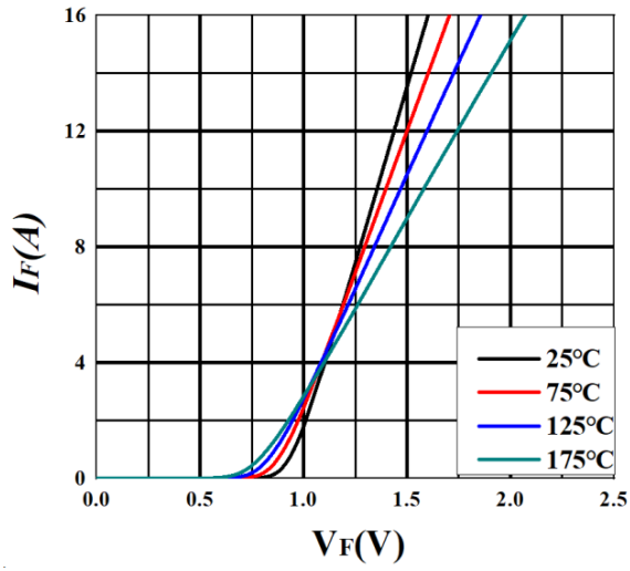
Figure 1. Forward characteristics
