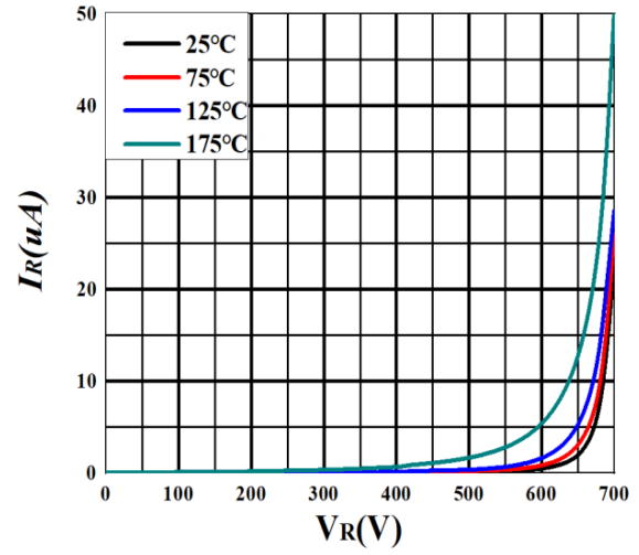
Figure 2. Reverse characteristics
