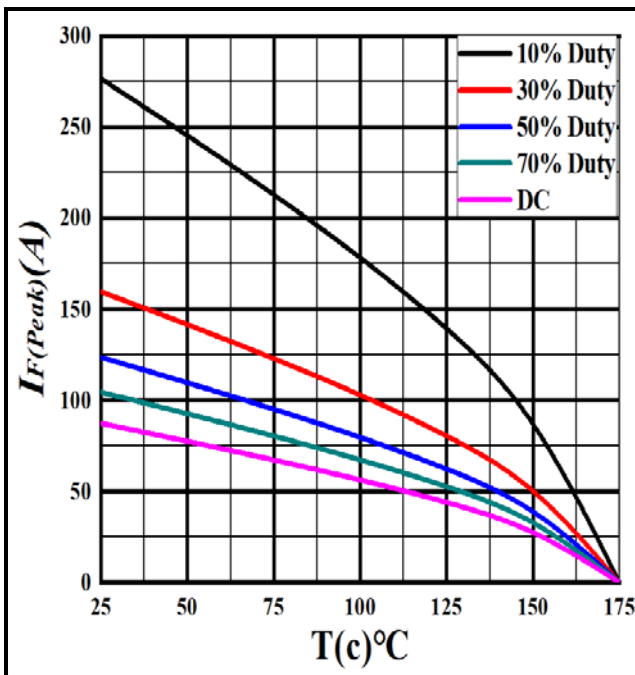
Figure 3. Current derating
