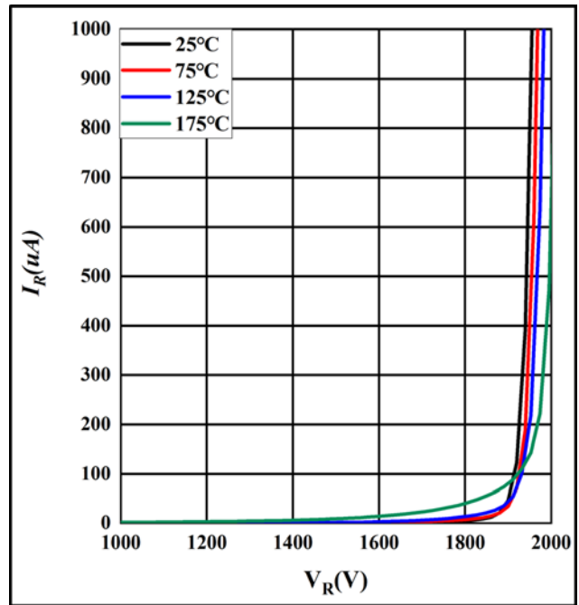
Figure 2. Reverse characteristics
